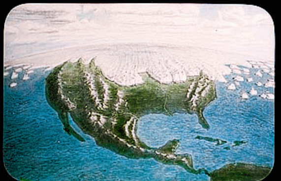
GLACIAL PERIOD—GENERAL VIEW
